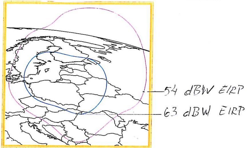
Figure A3-3-2-5: Transmit Enhanced Offer Area and Service Area for the Polish beam (2170-2200MHz)
