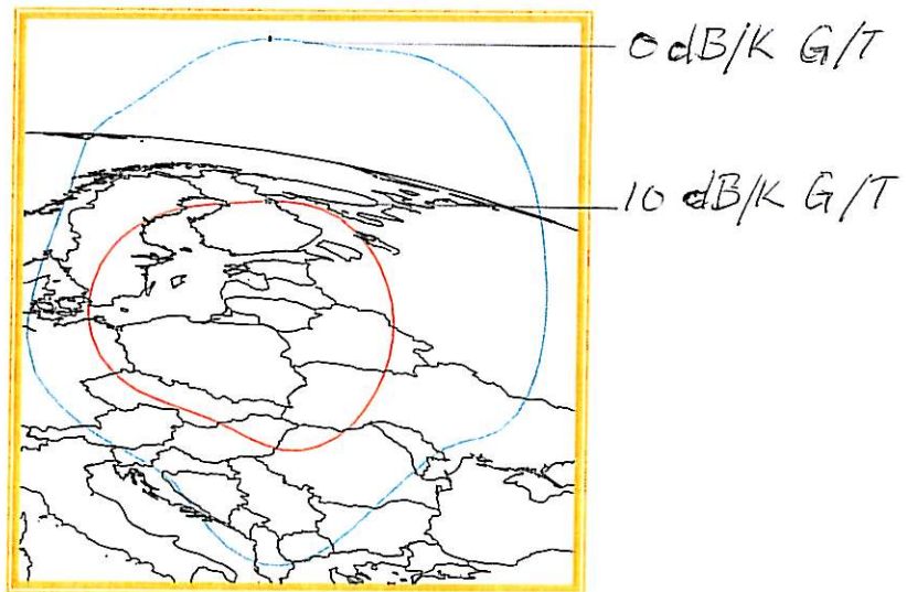
Figure A3-3-2-6: Receive Enhanced Offer Area and Service Area for the Polish beam (1980-2010MHz)
